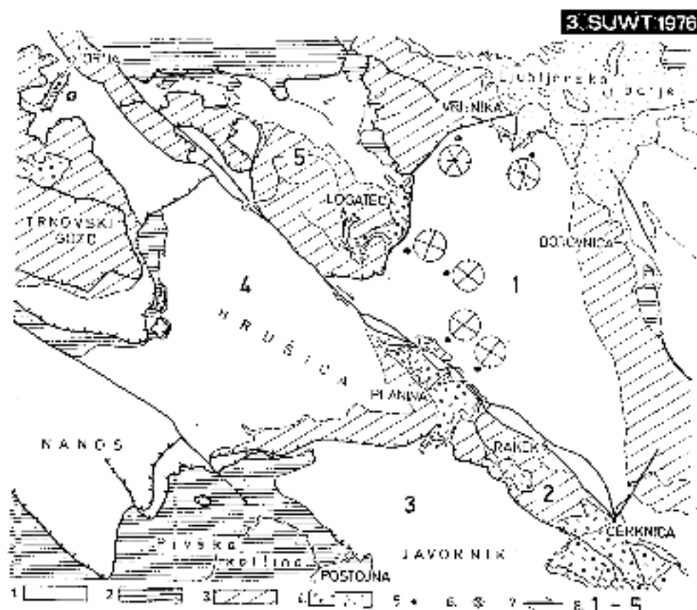
Fig. 5. Hydrogeologic units in the central part of Ljubljana Karst river basin. 1 — limestone, 2 — impermeable rocks (schists, etc.), 3 — dolomite, 4 — sediments on the karst paljes and moor, 5 — location of rupture survey, 6 — rupture diagrams, simplified, 7 — Idrija wrench fault (7) and other faults, 8 — hydrogeologic units: (1) — Vrhniko-Cerknica block, (2) — Rakov-Cerknica imbricate structure, (3) — Javorniki-Snežnik block, (4) — Hrušica block, (5) — Idrija-Ziri nappes area (all after S. BUSER 1965).
