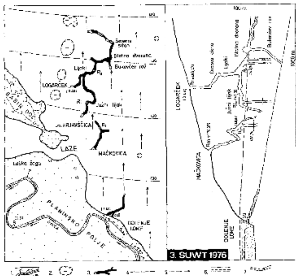
Fig. 18. The situation and cross section of caves at eastern Planinsko polje border. 1 — karst polje's border with superficial river bed and swallow-holes, 2 — collapsed dolines, 3 — simplified caves ground plan, 4 — lowest known karst water level — hydraulic contour lines, 5 — direction of karst water outflow, 6 — the floods altitude on polje and in caves, 7 — the pools of caught water in the cave, simplified cave's cross section.
