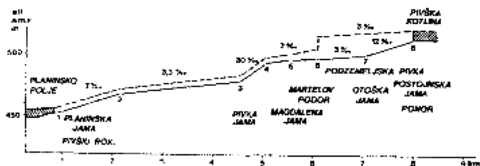
Fig. 8. Low and high water gradients between Pivka basin and Planina polje
