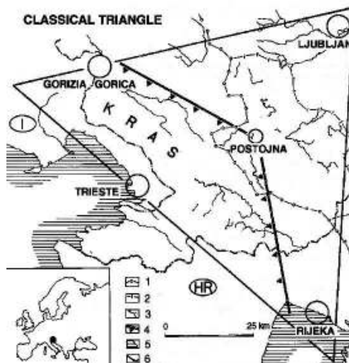
Fig. 2. The Classical Karst Triangle.
