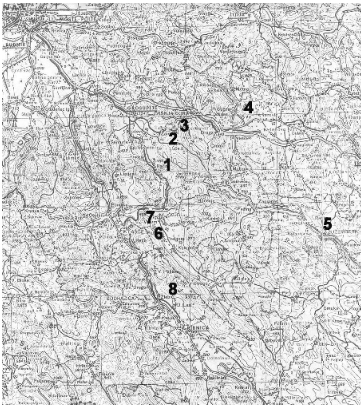
Fig. 14. The plan for the excursion on Friday, June, 28 th
