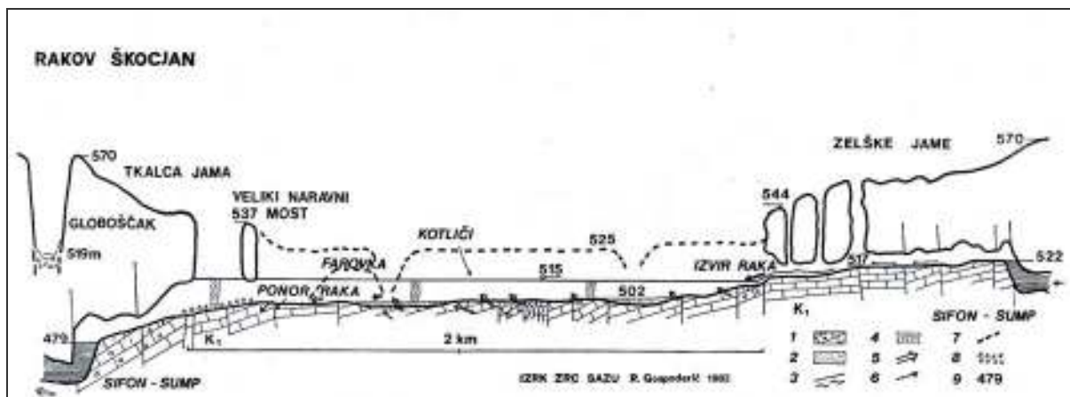
Fig. D4: Cross-section along Rakov Škocjan karst depression between spring at Zelške jame and sink in Tkalca jama. Legend: 1 – rocky bottom, 2 – alluvia, 3 – fault zone, 4 – flood in 1982, 5 – karst spring, 6 – water flow directions, 7 – terraces, 8 – boulder rocks, 9 – altitude (Gospodarič et al. 1983)
