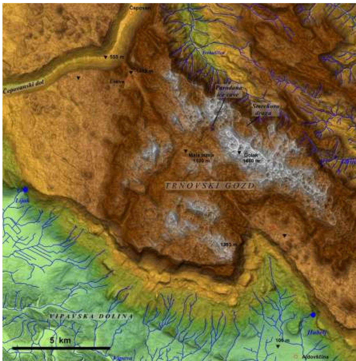
Fig. C5: DEM of the central part of Trnovski gozd karst plateau. Dry valley Čepovanski dol separates it from another plateau on NW.
