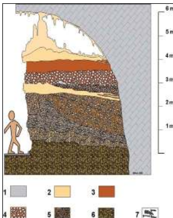
Fig. A4: Schematic cross section of the sediment profile at the entrance part of the Rov novih podpisov passage. Legend: 1. limestone, 2. flowstone, 3. cave loam and clay, 4. limestone rubble mixed with clay, 5. rubble and breccia, mostly of broken flowstone, 6. flysch gravel and clay, 7. bones of a cave bear.
