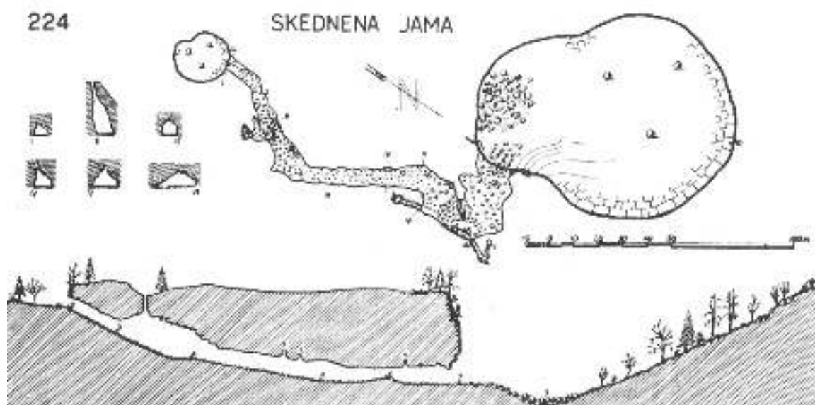
Fig. B3: Cross section through Skednena jama.
