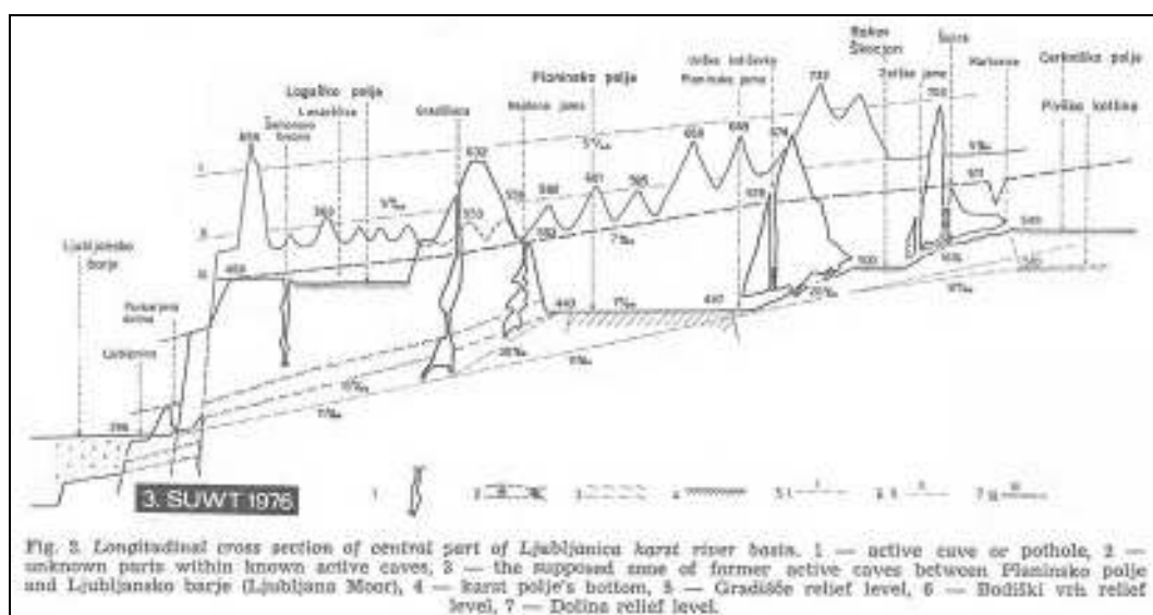
Fig. D3: Longitudinal cross section of Ljubljana karst river basin (Gospodarič & Habič 1976).
