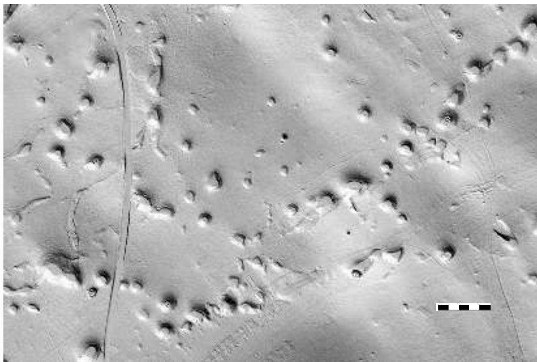
Fig. E14: LIDAR image of dolines and unroofed caves on Podgorski kras plateau (0.5 m grid). The scale bar is 100 m.
