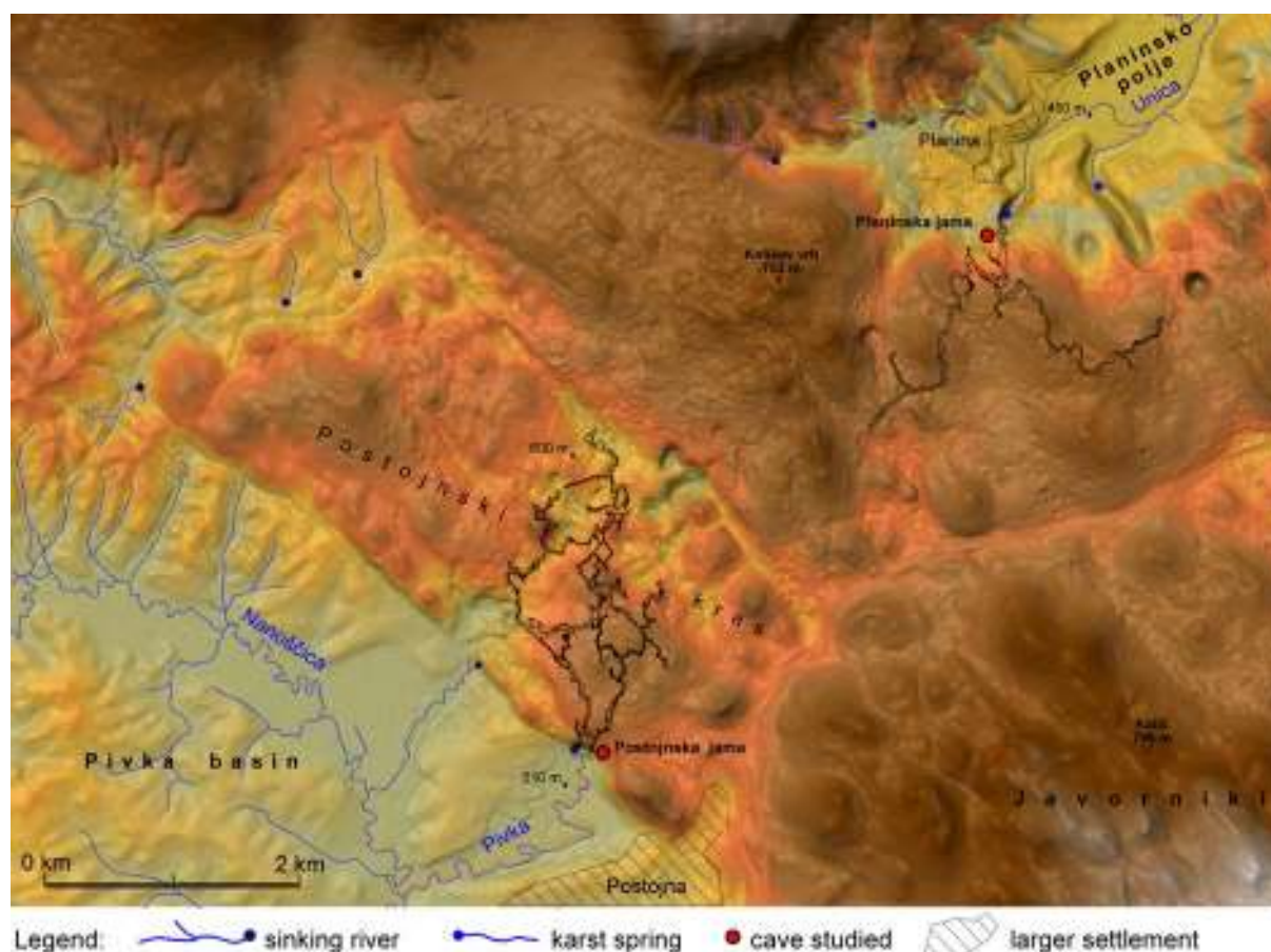
Fig. A1: Map of the karst between Pivka basin and Planinsko polje with cave system Postojnska jama – Planinska jama.
