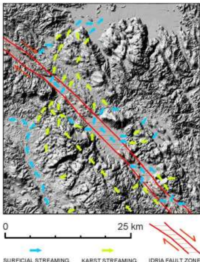
Fig. D2: Influence of the Idria Fault zone upon the karst poljes hydrology
