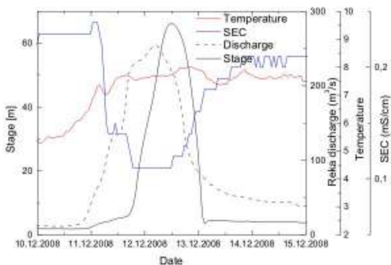
Fig. E10: Discharge, stage, temperature and SEC of Reka during the flood event in December 2008. Discharge is measure at the gaging station about 6 km upstream from Škocjanske jame.
