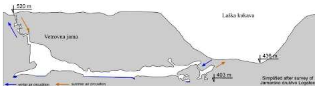
Fig. B5: Schematic cross section through Vetrovna jama and Laška kukava.
