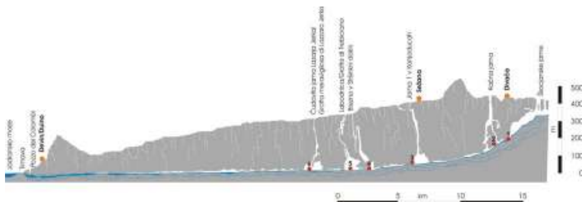
Fig. E8: Simplified cross-section of the Kras plateau with main caves and measurement points.
