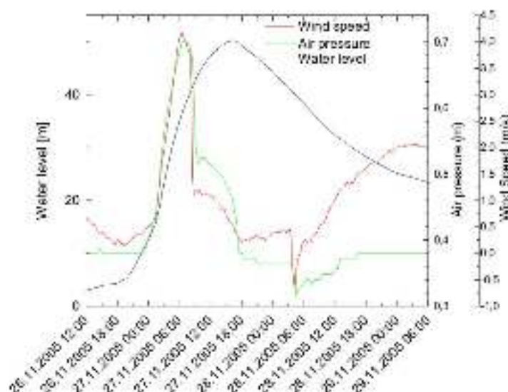
Fig. E.12: Water level, air pressure and wind speed during the flood event in November 2005.
