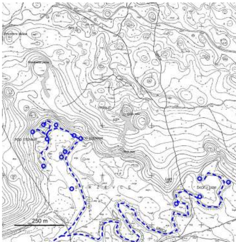
Fig. B2: Topographic map of N edge of Planinsko polje. Skednena jama and Vranja jama are marked. Unica here disappears in numerous swallow holes in alluvium.
