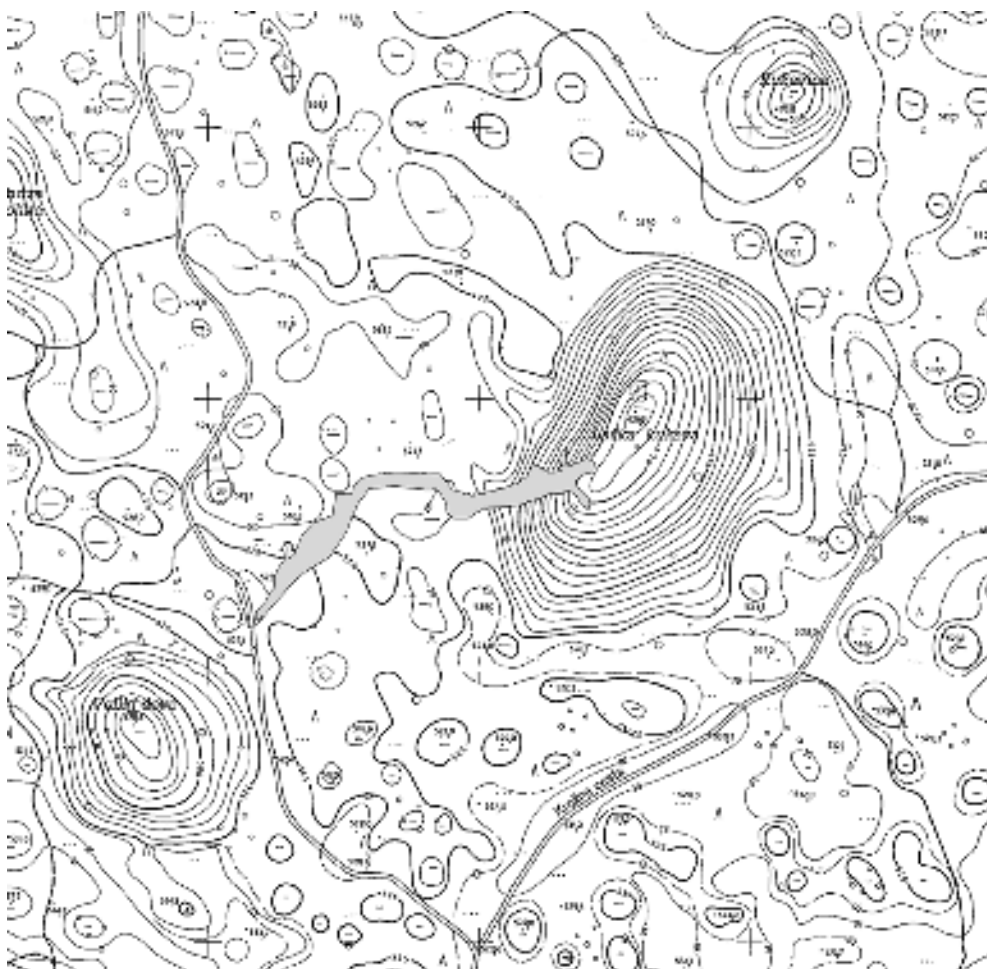
Fig. B4: Topographic map of Laška kukava and the position of the cave. In some other large collapse dolines the summer temperature inversion is also maintained by the cold cave air.
