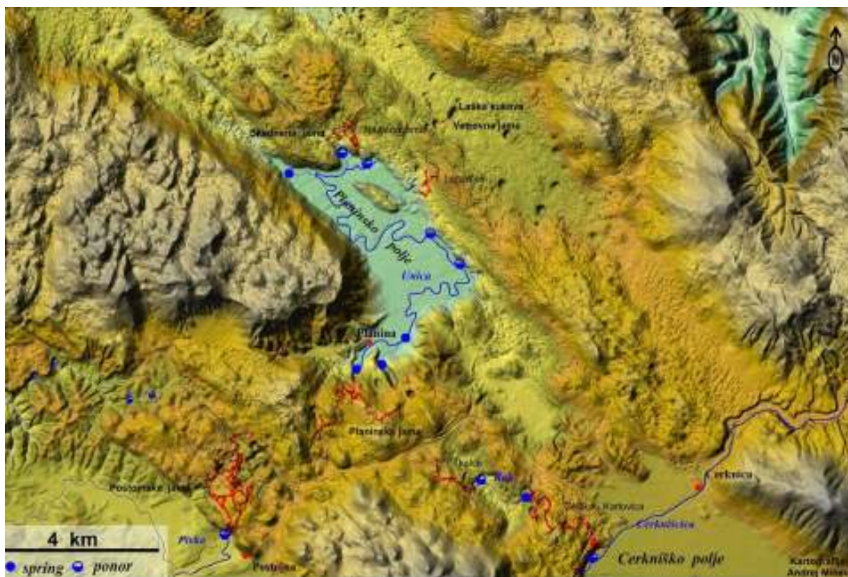
Fig. B1: Planinsko polje and adjacent karst.
