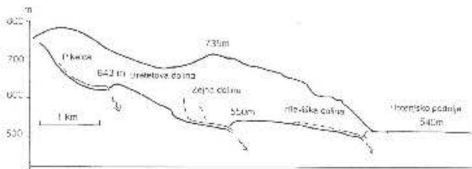
Fig. D5: Schematic cross section trough active valleys of three sinking brooks Pikelce, Žejnski potok and Hlevišarka and dry valleys in between to Hotenjsko polje.
