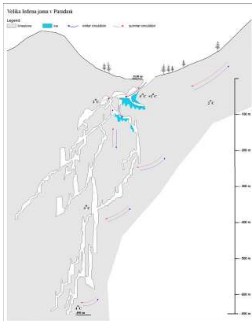
Fig. C6: Schematic cross section and some climatic observations from the Velika ledena jama v Paradani.
