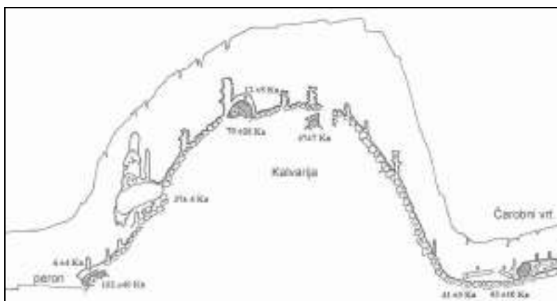
Fig. A3: Schematic cross section trough Kalvarija (Velika gora) collapse. Positions of samples and the age of the flowstone are marked on the sketch.
