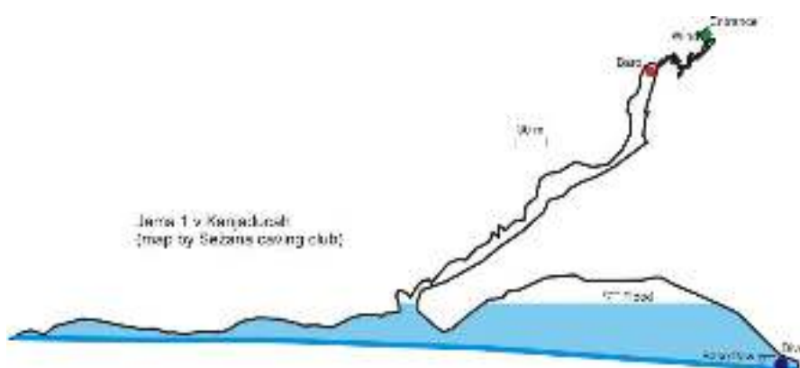
Fig. E.11: Extended elevation of Jama 1 v Kanjaducah with the positions of instruments.
