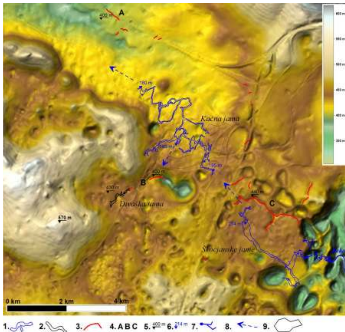
Fig. E4: The map of the Divača karst. On the levelled surface the large collapse dolines are dominating features, solution dolines are frequent, but they represent only small proportion of the surface. The outlines of the main caves and the main unroofed caves are marked. On the map made of DEM with 12.5 m grid the road cuts or causeways are also seen.
