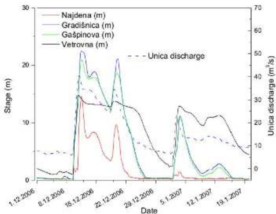
Fig. B6: Stage response to a flood in caves Ne from Planinsko polje. Note the delayed recession in Vetrovna jama.
