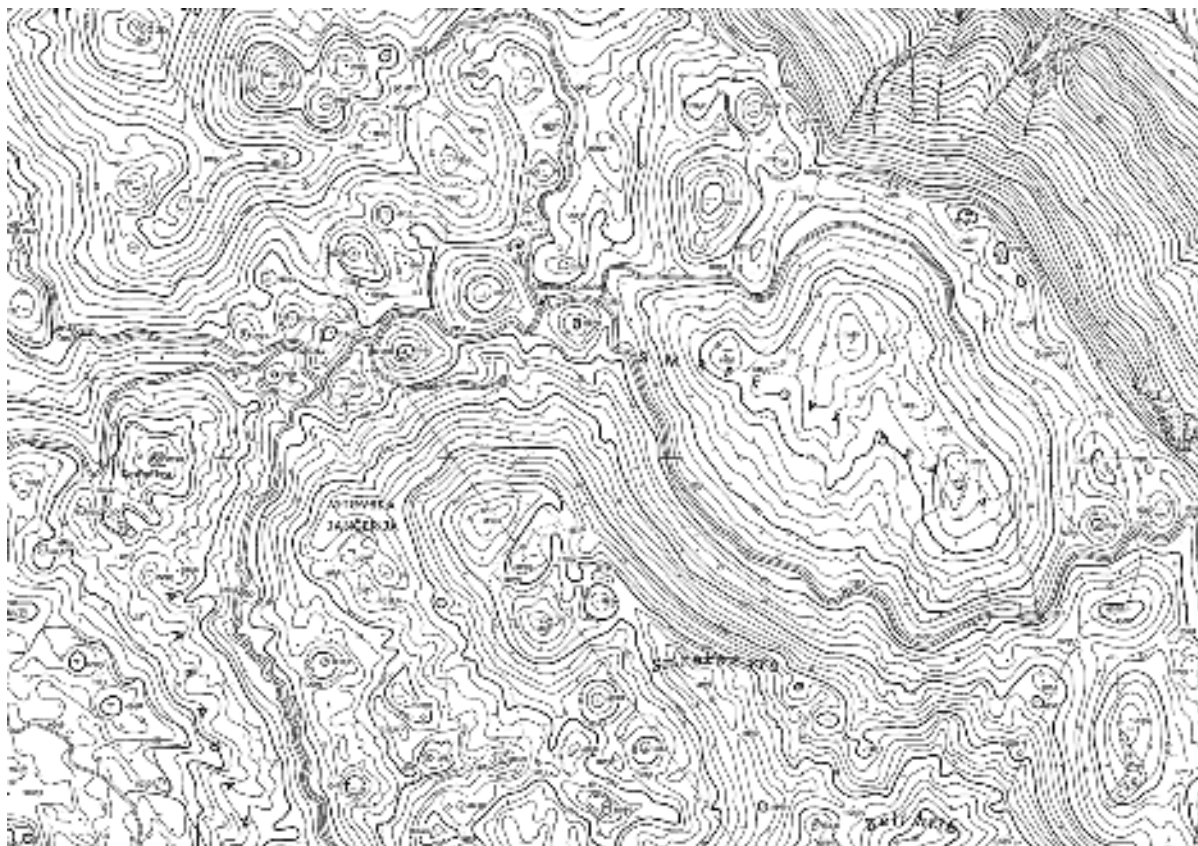
Fig. C4 : Topographic map of central part of Trnovski gozd with numerous large dolines.
