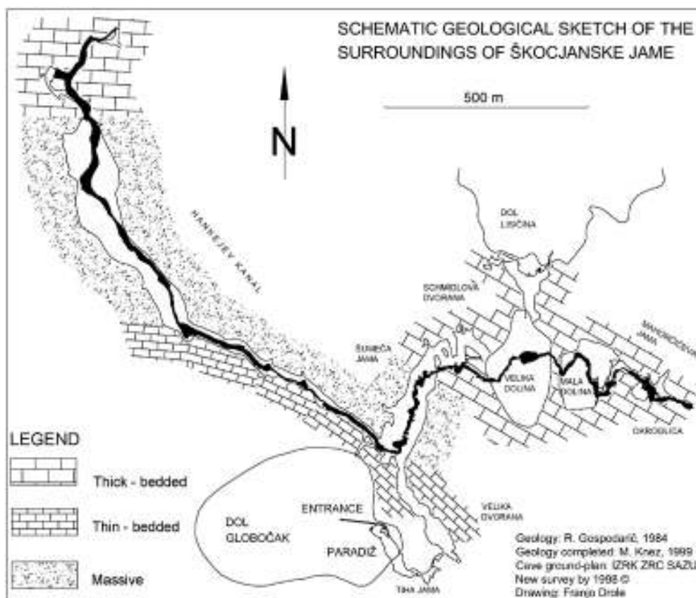
Figure 1. The geological map of the Škocjanske jame (Mihevc & Gabrovšek 2012).
