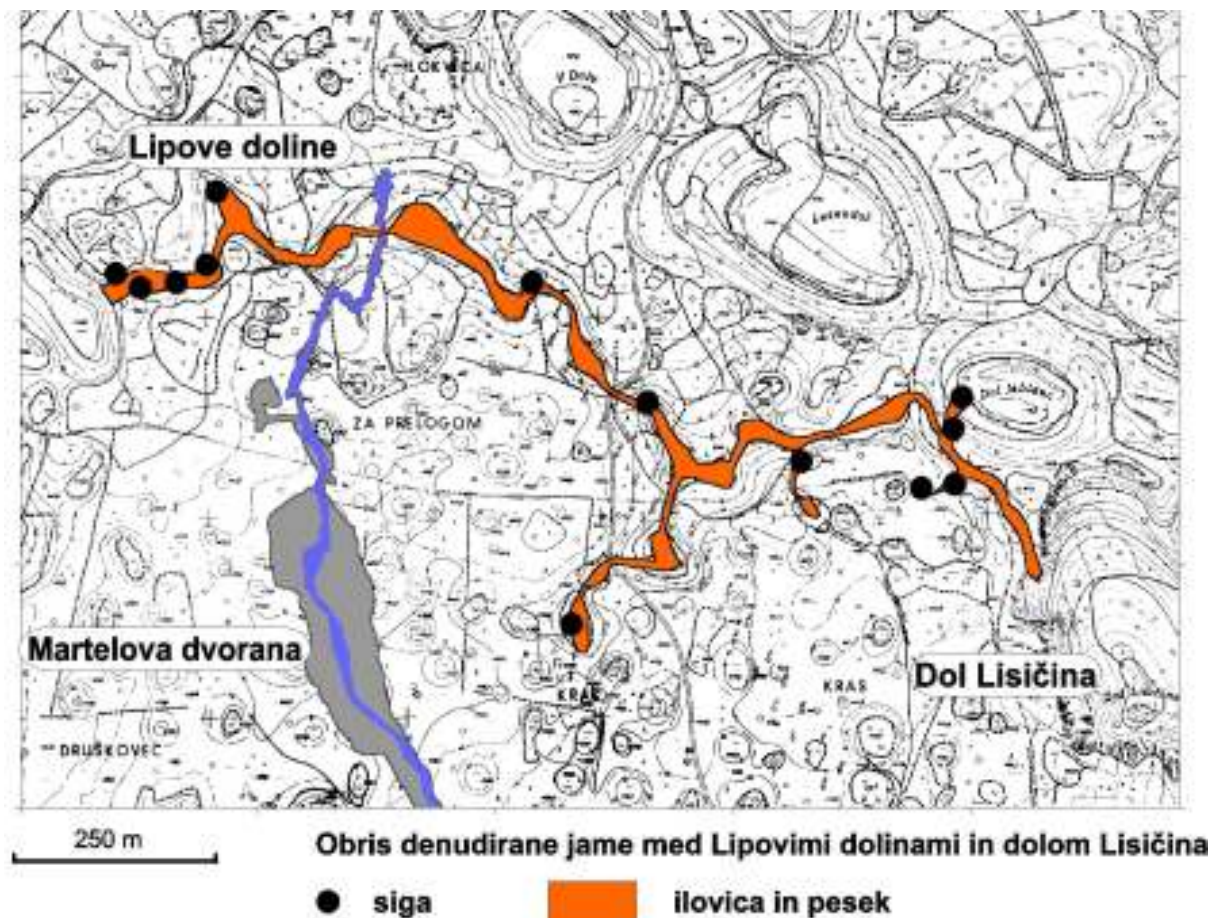
Fig. 3: Unroofed cave Lipove doline (Mihevc, 2001). The surface is between 420 and 440 m a.s.l. Black dots: outcrops of massive flowstone; orange colour: outline of the cave sediments; grey outline: the extreme N part of Škocjanske jame; blue outline: river Reka between 220 m and terminal sump at 190 m.a.s.l.
